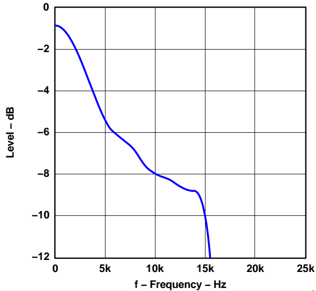
DE-EMPHASIS FREQUENCY RESPONSE (32 kHz)
