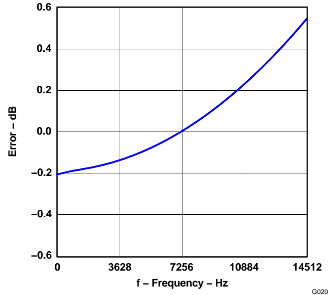
DE-EMPHASIS ERROR (32 kHz)
