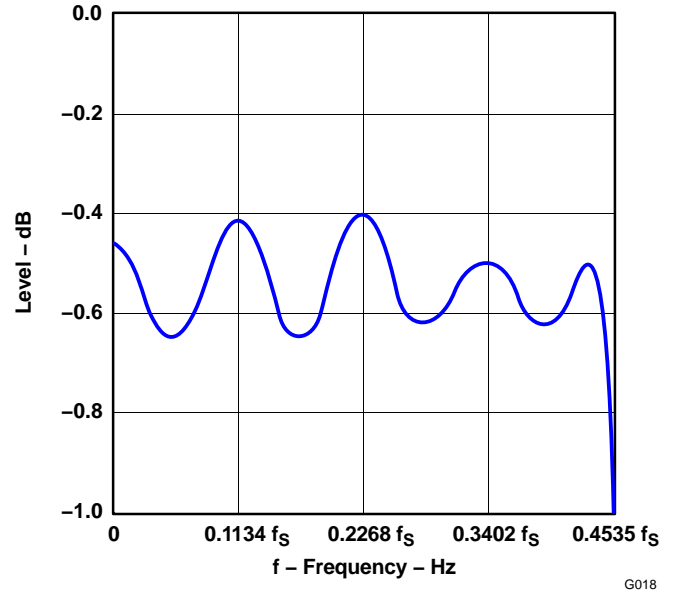
PASS-BAND RIPPLE CHARACTERISTIC
