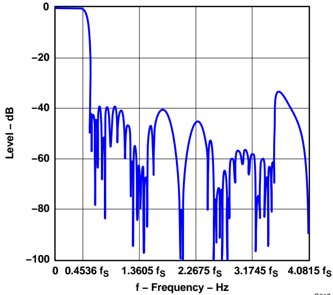
OVERALL FREQUENCY CHARACTERISTIC
